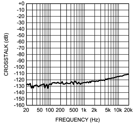
Crosstalk vs Frequency V_{CC} = 2.5V, V_{EE} = -2.5V, V_{OUT} = 1V_{RMS} A_V = 0dB, R_L = 10k\Omega
